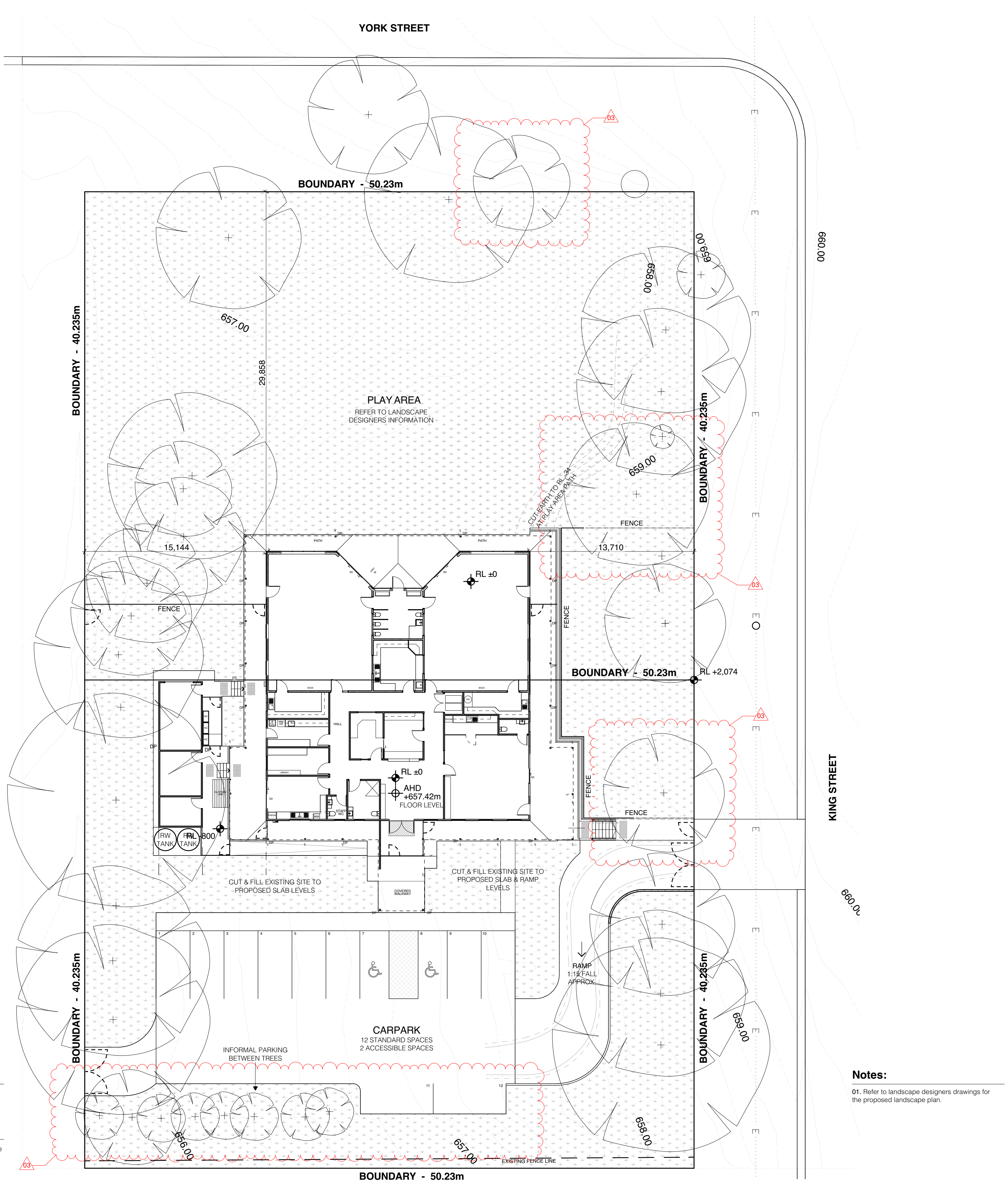
02 Site Plan - Proposed 1:200
